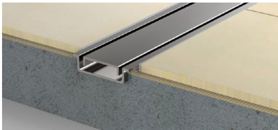
Drainage slotted channel for toilets and showers
